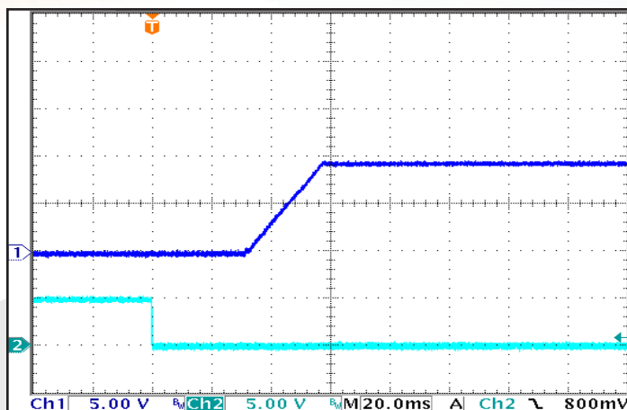
Figure 7: Typical Startup Waveform, input voltage pre-applied. Ch 1: V_{out} (5 V/div); Ch 2: ON/OFF Pin (5 V/div). Timescale 20.0ms/div.
