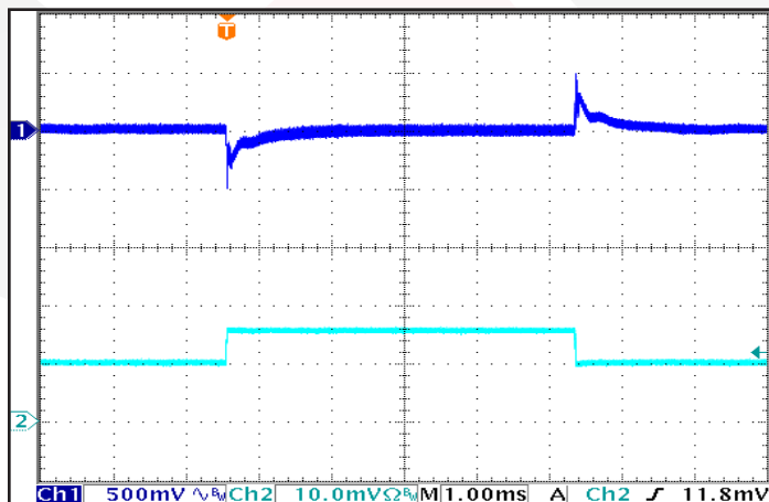
Figure 11: Output Voltage Response to Step-Change in Load Current, (50%-75%-50% of I_{out(max)} ; dI/dt = 5 \text{ A}/\mu\text{s} ). Load capacitance: 1 μF ceramic and 100 μF electrolytic capacitors. Ch 1: V_{out} (500 mV/div); Ch 2: I_{out} (20 A/div). Timescale: 1.00ms/div.
