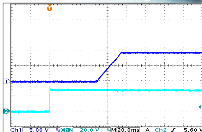
Figure 8: Turn-On Transient, at full resistive load and zero output capacitance, initiated by V_{in} . Ch 1: V_{out} (5 V/div); Ch 2: V_{in} (20 V/div). Timescale: 20.0ms/div.
