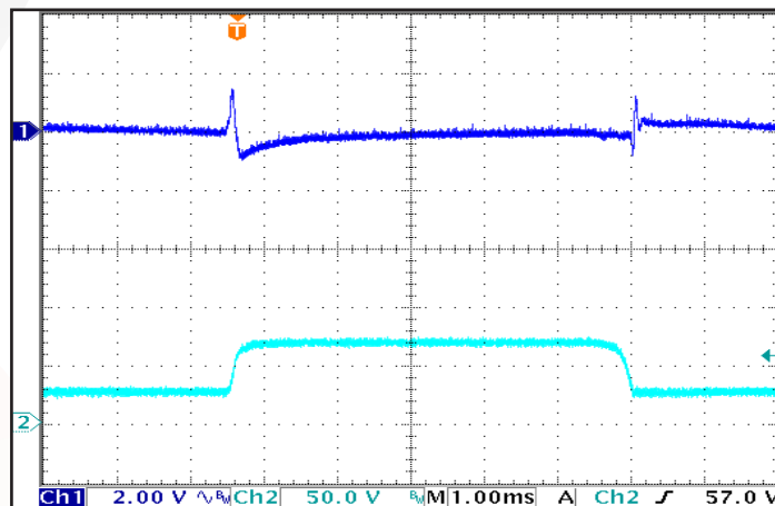
Figure 12: Output Voltage Response to Step-Change in Input Voltage, ( dV/dt = 250 \text{ V}/\text{ms} ). Load capacitance: 100 μF electrolytic capacitors. Ch 1: V_{out} (2 V/div); Ch 2: V_{in} (50 V/div). Timescale: 1.00ms/div.
