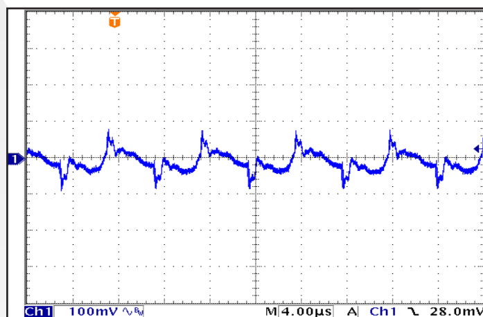
Figure 10: Output Voltage Ripple, V_{out} , at nominal input voltage and rated load current (100 mV/div). Load capacitance: 1 μF ceramic and 100 μF electrolytic capacitors. Bandwidth: 20 MHz. Timescale: 4.00μs/div. See Figure 13.
